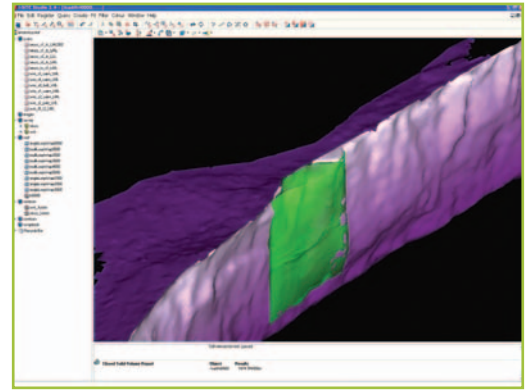
Modelled data of glacier icefall
