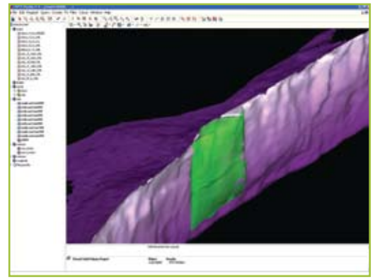
Modelled data of glacier icefall
