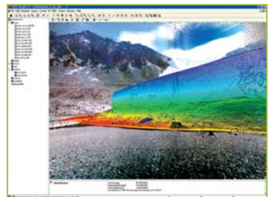
Scan data of Sues glacier
